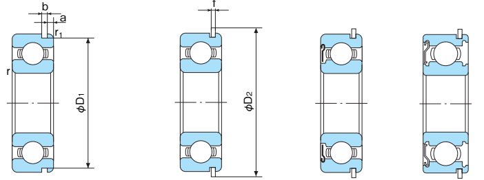
With snap ring groove (N) With snap ring (NR) Shield type with snap ring (ZNR) Shield type with snap ring (ZENR)
